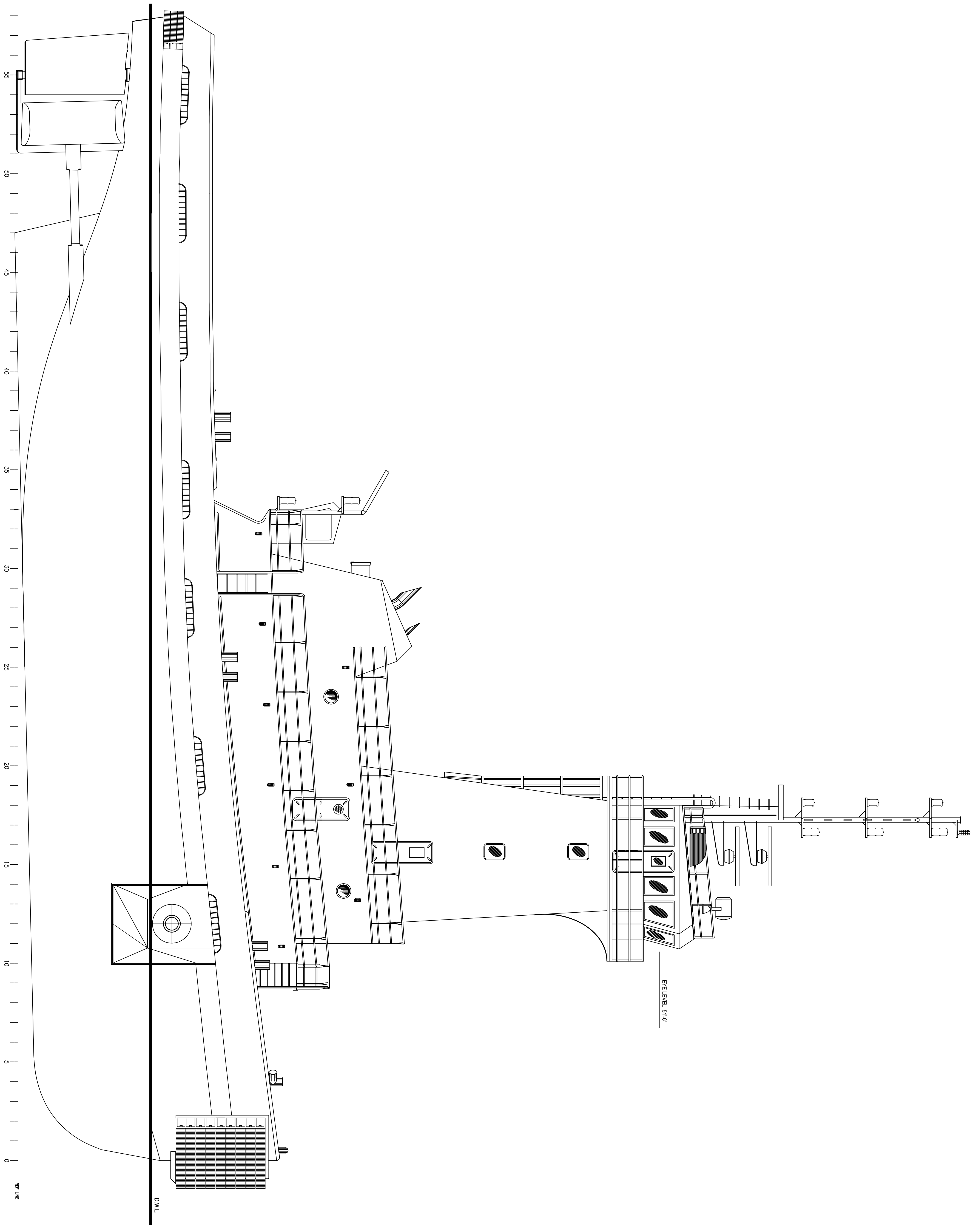
OUTBOARD PROFILE
